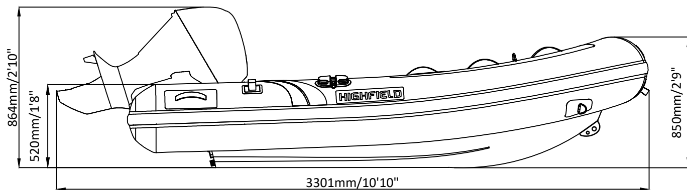
Side View
